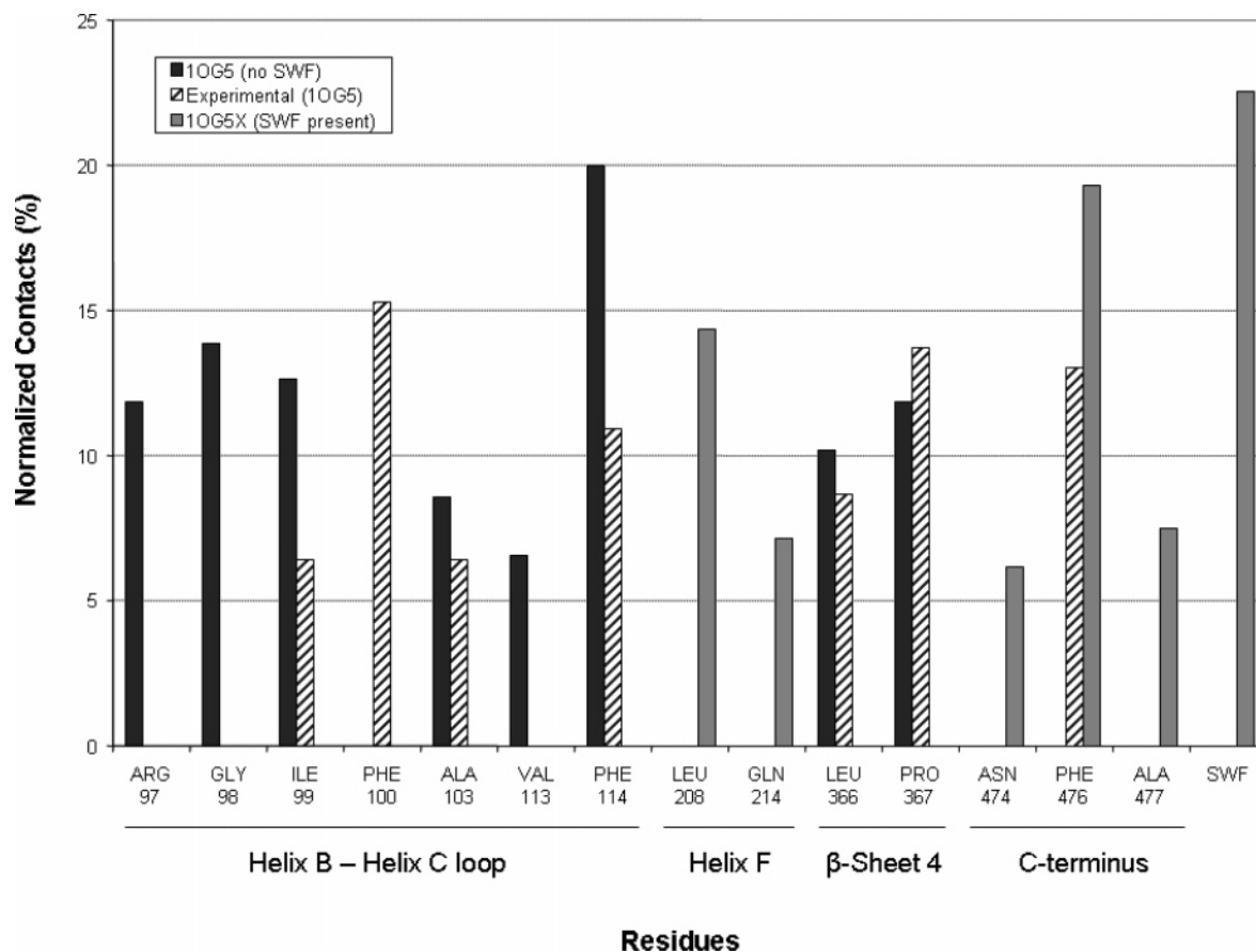
FIGURE 7: Distribution of normalized intermolecular nonbonded contacts for P450 2C9 structures. The mapping results are based on the interactions found between the probes in the consensus site and the residues of the protein. The interactions are normalized on the basis of the total number of interactions for each mapping result, and only residues making at least 5% of the total contacts are shown (see Materials and Methods). The best consensus site is considered for the S-warfarin-bound P450 2C9 structure 1OG5, without ligand present (1OG5) and with ligand present (1OG5X). The nonbonded contacts for S-warfarin in the bound structure 1OG5 are obtained from the database PRECISE (see Materials and Methods) and are shown for comparison to the mapping results. The structural references below the residues were included to help in orientation of the interactions within the binding pocket. SWF denotes the intermolecular contacts found between the probes and S-warfarin for 1OG5X, where S-warfarin was retained as part of the protein. The figure shows the union of the three distributions of interactions determined for P450 2C9.
